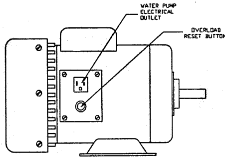
Electric Motors With Overload Protection
